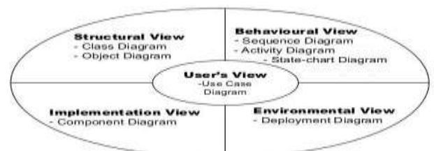
Figure 1: UML Diagrams
