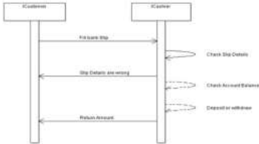
Figure 7: Sequence diagram
